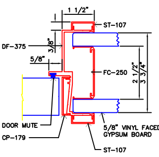
15 DOOR JAMB AND HEADER SOLID PARTITION
