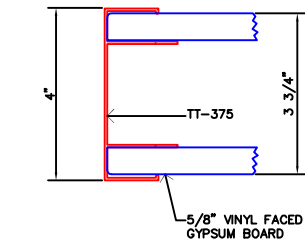
19 FINISHED END / TT-375
