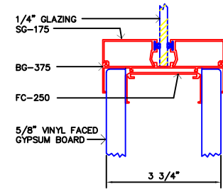
4 SILL / GLAZING
