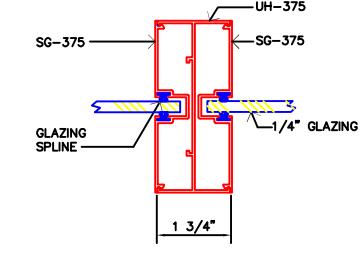
20 GLAZED MULLION
