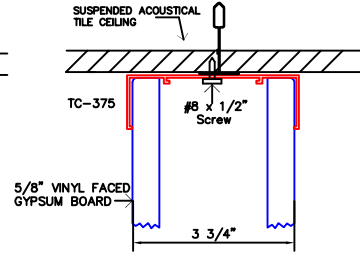
6 CEILING HEAD CONDITION
