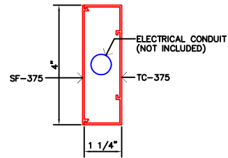
3 THROUGH POST
