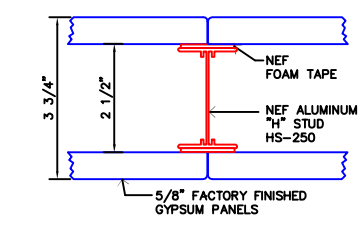
13 PARTITION JOINT/NEF ALUMINUM "H" STUD
