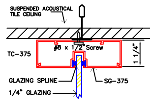
8 GLAZED HEAD AT CEILING
