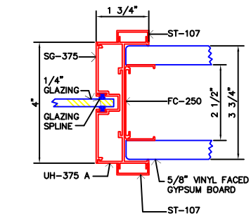
24 TRANSITION TO GLASS PANEL
