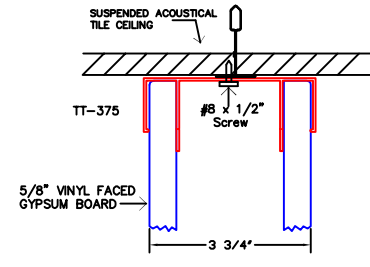
5 HEAD CONDITION FULL OR RAIL HEIGHT
