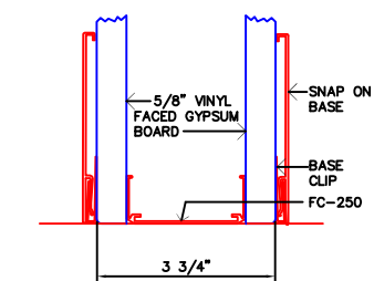
12 FLOOR CONDITION CLIP ON BASE W/ CLIP
