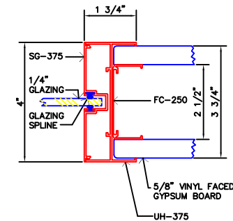
23 TRANSITION GLASS TO PANEL
