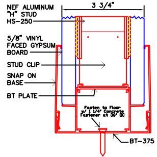
10 FLOOR CONDITION STUD WITH STUD CLIP
