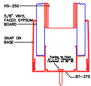
9 FLOOR CONDITION
