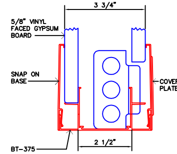
11 FLOOR CONDITION INTEGRAL CLIP ON BASE
