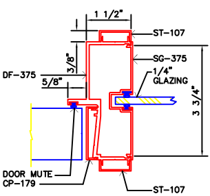
22 DOOR FRAME WITH GLASS TRANSITION
