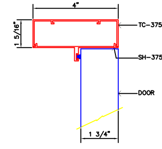
7 FULL HEIGHT DOOR FRAME WITH STANDARD SNAP HEADER
