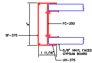
18 FINISHED END / UH-375
