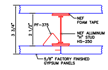
14 PARTITION JOINT/NEF ALUMINUM "H" STUD WITH NON-PROGRESSIVE EDGE CLIP STAGGERED JOINT
