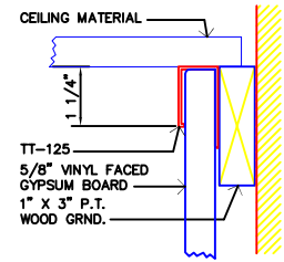
1 PANEL ON WOOD FURRING
