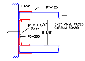
17 TERMINATION
