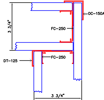
16 OUTSIDE CORNER
